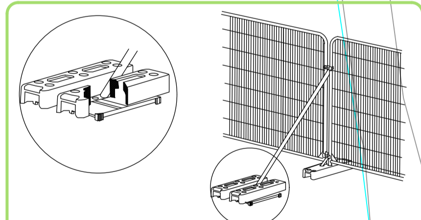
ILLUSTRATION SHOWING HERAS FENCING AS TEMPORARY GROUND/ROOT PROTECTION BARRIER WITH STABILIZER MOUNTED ON BLOCK TRAY ON ROOT SIDE AS RECOMMENDED BY BS 5837:2012 SEE PLAN FOR POSITIONING
